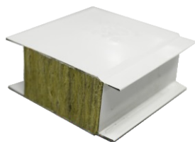
机制岩棉板 Mechanized rock wool board
